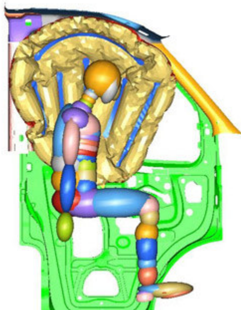
Delphi Side Curtain Airbag Module
